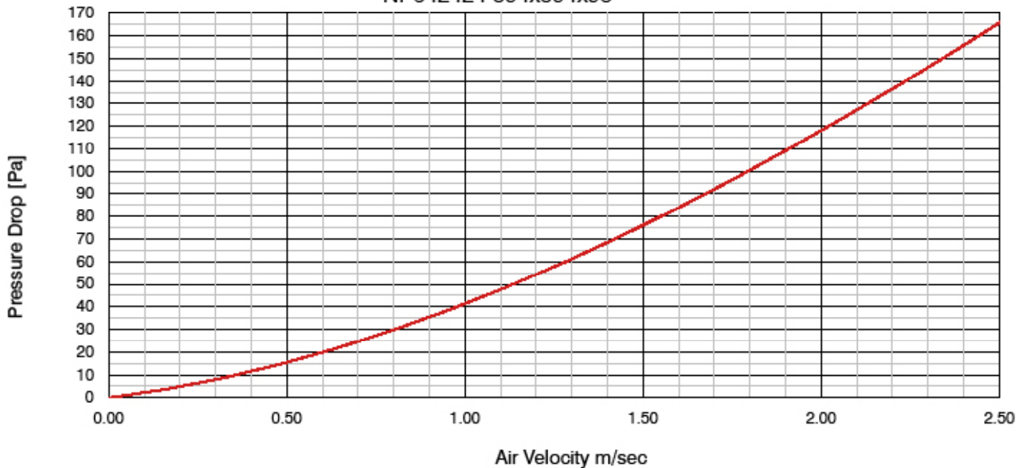
Pressure drop (Pa) Vs Velocity (m/sec) NP642424 594x594x95
